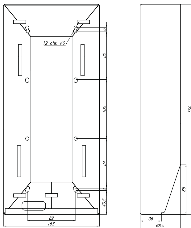
Figure 29: Dimensions of panels CP-2520 and panels NP2522, NP2521
